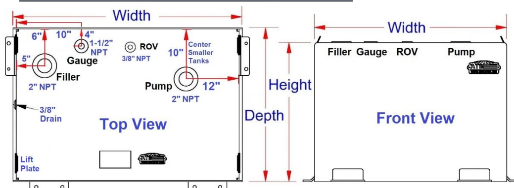
Steel Tank
